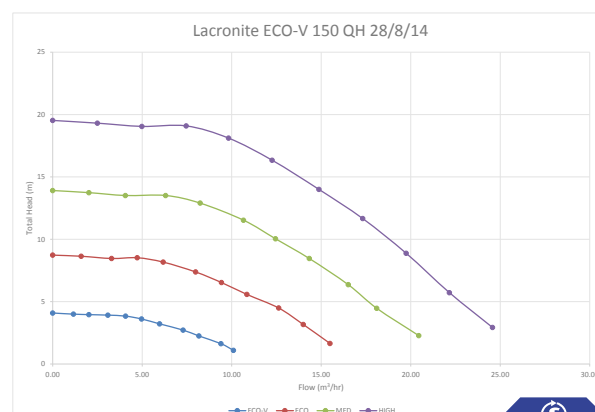
Flow Curve 150
