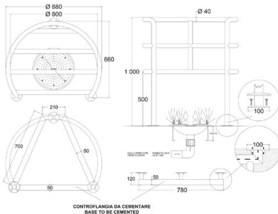
75213 Hydro Station With Seat Combination
