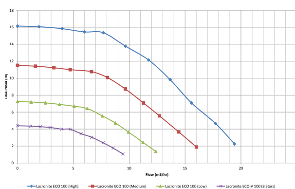
Flow Curve 100
