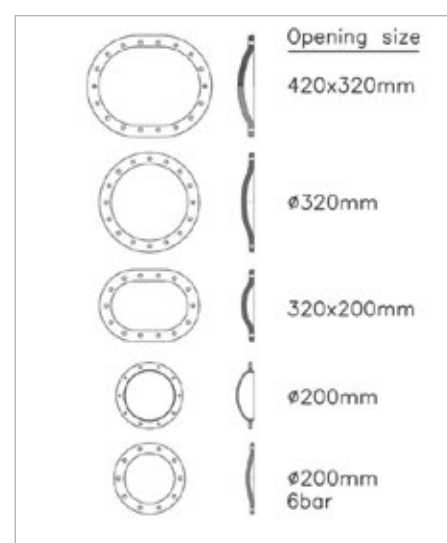
Side hatch/Lateral manhole covers
