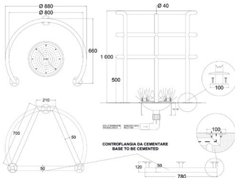
75210 Hydro Station Combination
