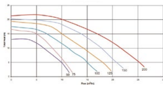
Flow Curve 100
