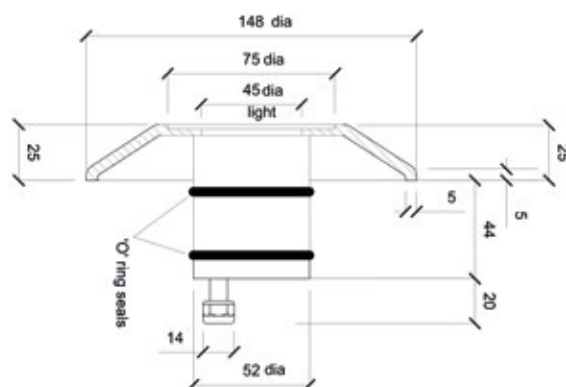
Push-fit 2" - pipe
